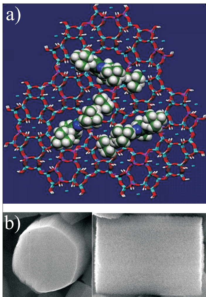
Fig. 5. a) Top view of a Van der Waals model of metal complex stopcock molecules (IL-1) reversibly adsorbed at the channel entrances of zeolite L. b) SEM images showing the morphology of zeolite L crystals ( left : bottom face of a crystal; right : coat of the crystal).
