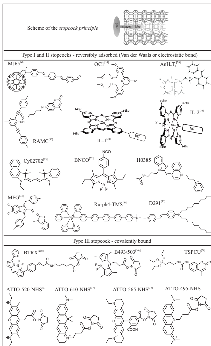
Fig. 4. Stopcock molecules
