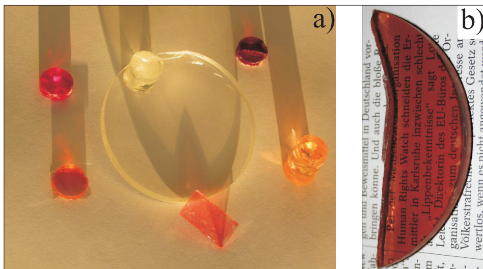
Fig. 7. Photographic images of transparent polymer-zeolite L hybrid materials. a) Selection of transparent dye-loaded and unloaded zeolite L-polymer hybrid materials. b) 1% wt/wt material prepared from Ox, HY3G-zeolite L.
