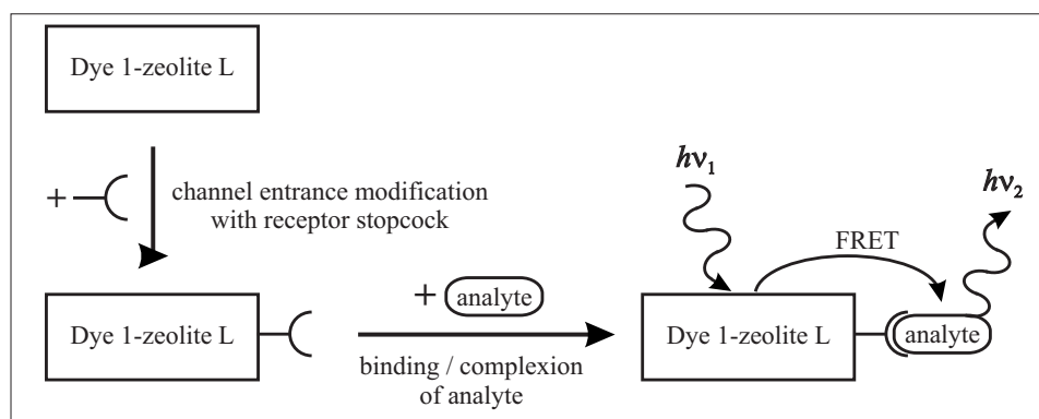
Scheme. Working principle of a functional energy transfer label . In a first step, the channel entrances of zeolite L crystals, loaded with Dye 1, are modified with a receptor stopcock. [27,41] The resulting material can now bind to a compatible analyte, so that the distance between Dye 1 and the analyte is short enough for energy transfer to occur.
