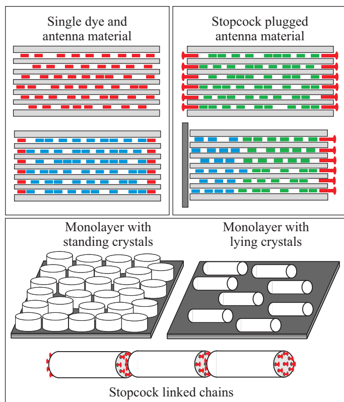
Fig. 1. Schematic representations of materials fulfilling the criteria of different stages of supramolecular organisation. All materials shown here have been successfully prepared. Top left: Single dye and antenna materials are obtained by either loading zeolite crystals with one kind of dye (top) or by the consecutive insertion of different dye molecules (bottom). Top right: Stopcock-plugged antenna material obtained by modifying either bidirectional (top) or monodirectional (bottom) antenna materials with specific closure molecules, called stopcocks. Bottom: Organisation of zeolite L crystals . Oriented monolayers of either standing or lying zeolite L crystals on a substrate and a chain of crystals linked by the interaction between the stopcocks located at the channel entrances.
