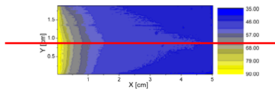
Figure 4: LBIC scan of a fluorescent concentrator with a solar cell attached to one side, a white bottom reflector and a photonic structure on top.
